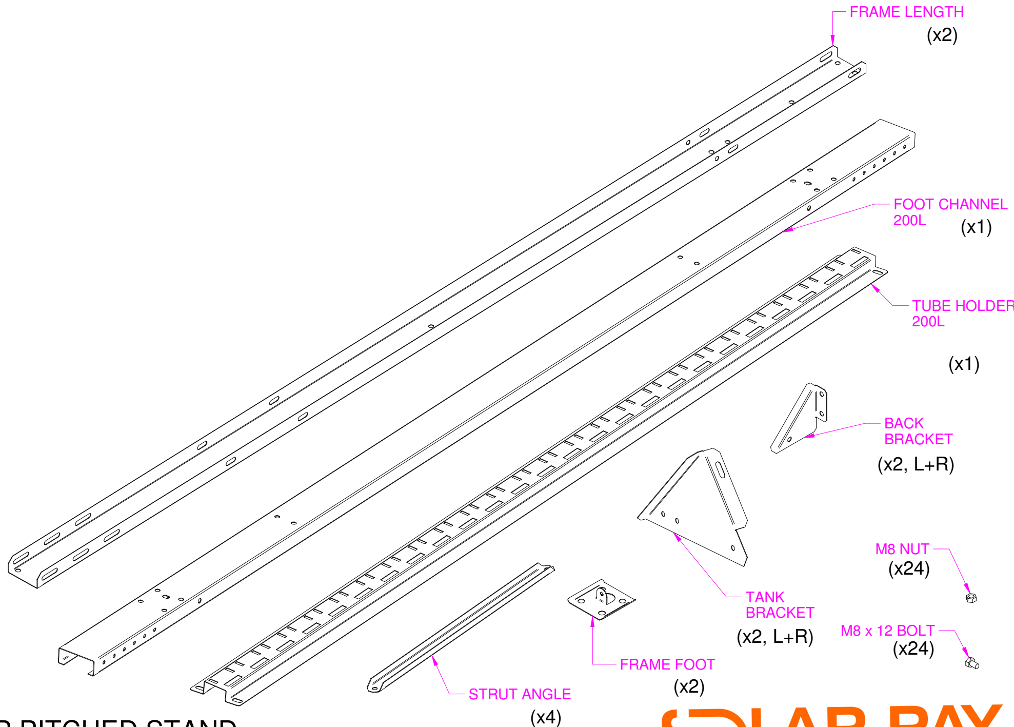
200L HP PITCHED STAND
